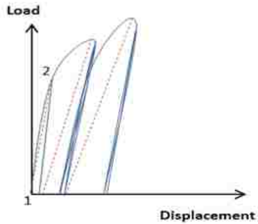
Figure 11. The procedure adopted for determining secant stiffness
