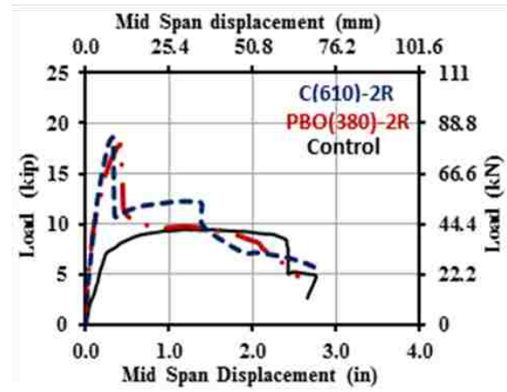
(b) Effect of type of fiber (FRCM)
