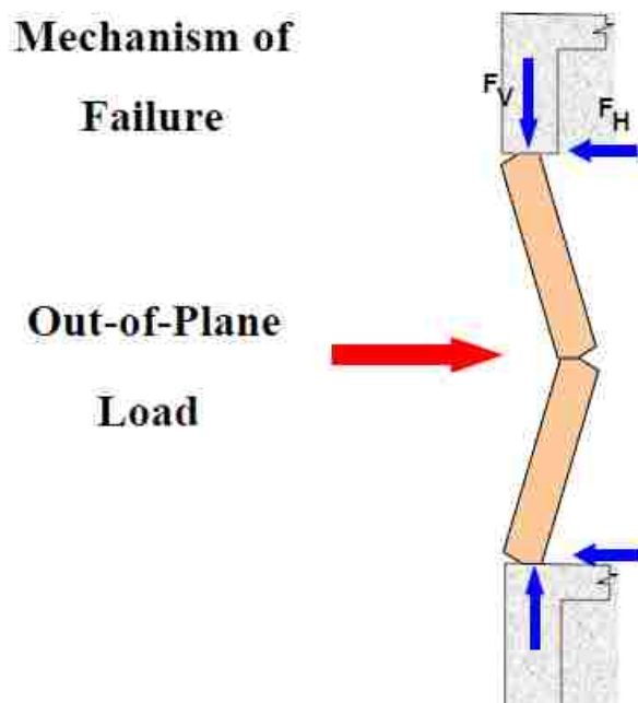
Figure 2.1. Arching Action Mechanism (Tumialan et al., 2001)
